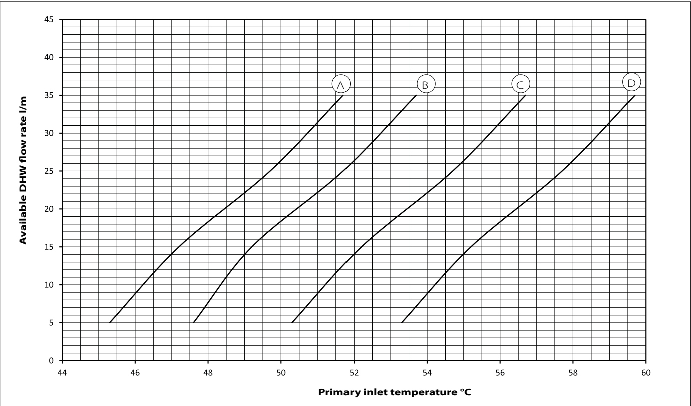
Quantity of water produced in l / m at different storage temperatures and different withdrawal temperatures
