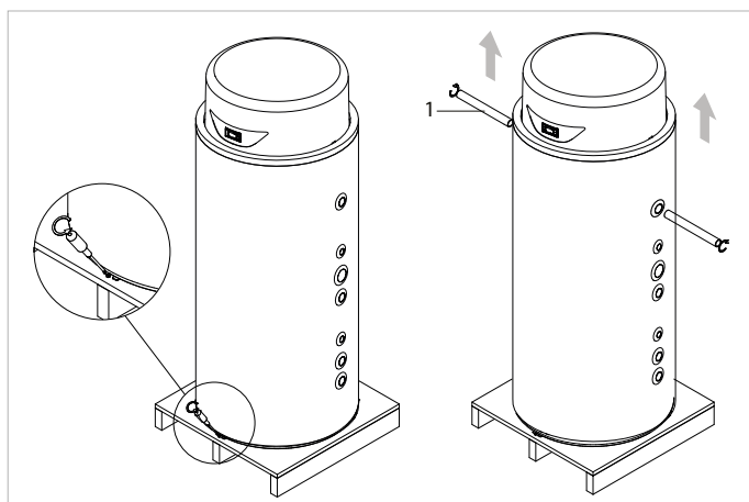
1. Threaded fitting
